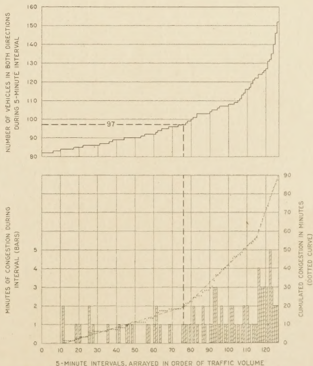
FIGURE 5.—DETERMINATION OF TRAFFIC CAPACITY OF 2-LANE ROADS, 60 PER CENT OF TRAFFIC IN ONE DIRECTION
